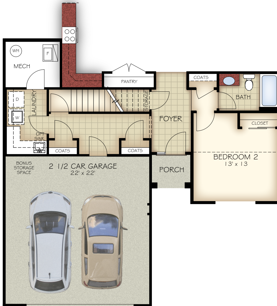
FIRST FLOOR PLAN WITH OPTIONAL BONUS SUITE
